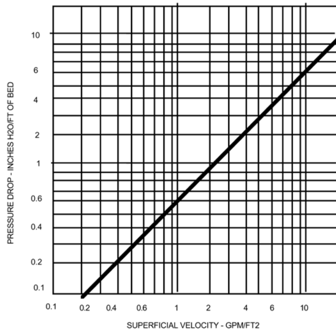
PRESSURE DROP vs VELOCITY 8 x 20 MESH
